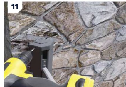
11: Using a 3mm drill bit, drill two pilot holes into the post, using the two predefined holes on the cap as a guide.
